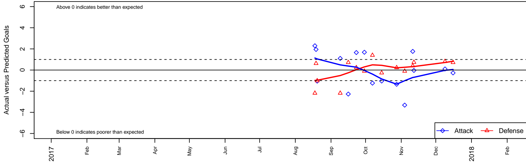
NWSC Deception FC G05 Dots are actual minus expected GF (blue circles) and GA (red triangles). Blue line is smoothed change in attack strength. Red is smoothed change in defense strength.
